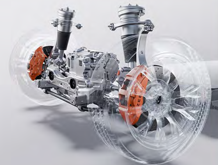
Akebono Front Four-piston Calipers
